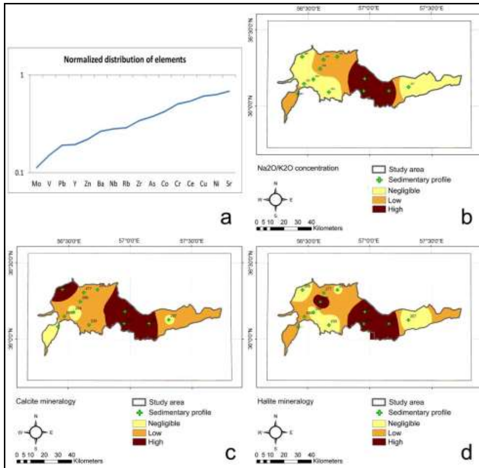
Figure (6): a. Normalized distribution of elemental enrichment plot, b. Geostatistical distribution of \text{Na}_2\text{O} , \text{K}_2\text{O} ratio, c. Geostatistical distribution of calcite mineralogy, and d. Geostatistical distribution of halite mineralogy
