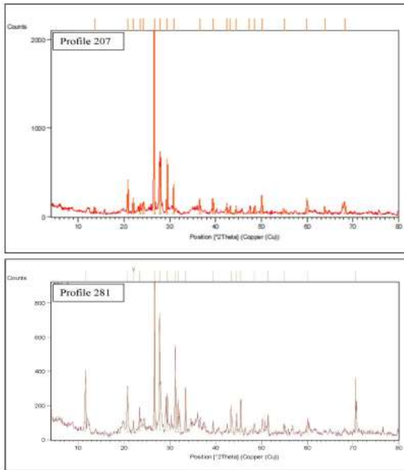
Figure (4): XRD patterns of some topo-soil samples in Sabzevar playa
