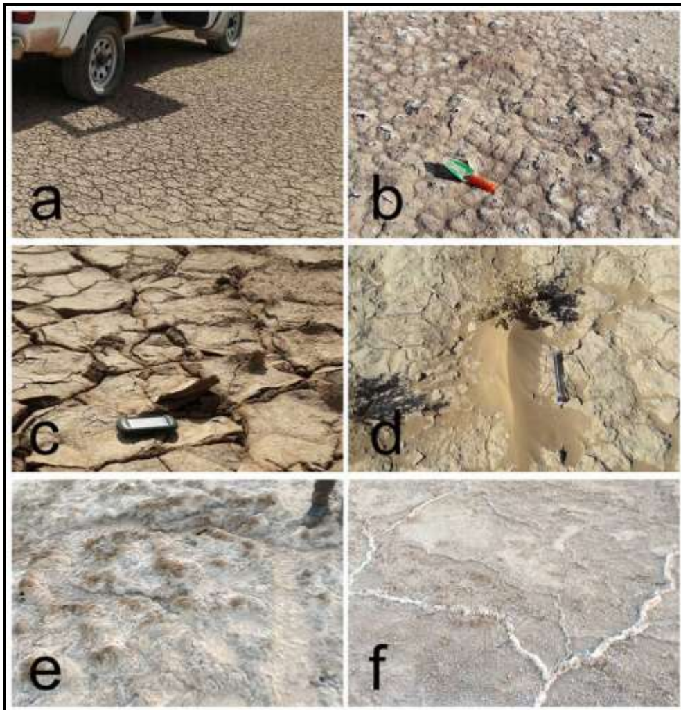
Figure (2): General vision of landforms consisted of firm-puffy ground (e, b), fine-clay ground and embryo Nebka (d), physical carbonate crust (a, c), and salt crusts, Takir (f)
