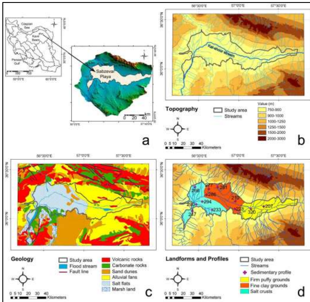
Figure (1): a. General position of the study area in great Kavir basin, central Iran, b. Topographical characteristics, c. Geological map, and d. General position of landforms and location of topo-soils
